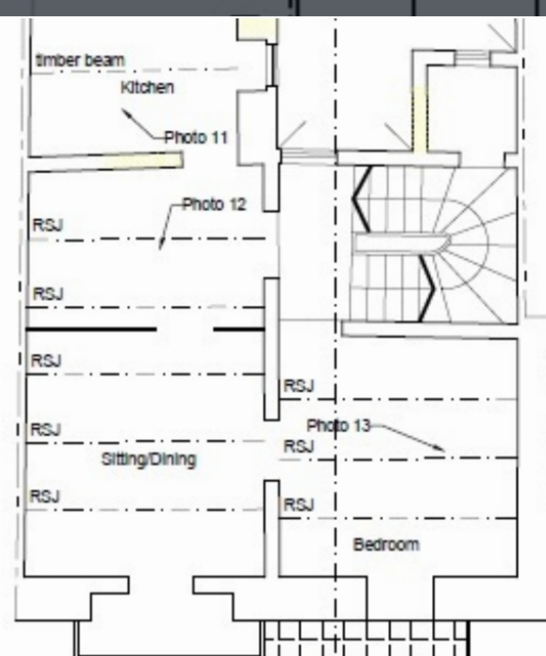
Existing Third Floor SCALE 1:100
