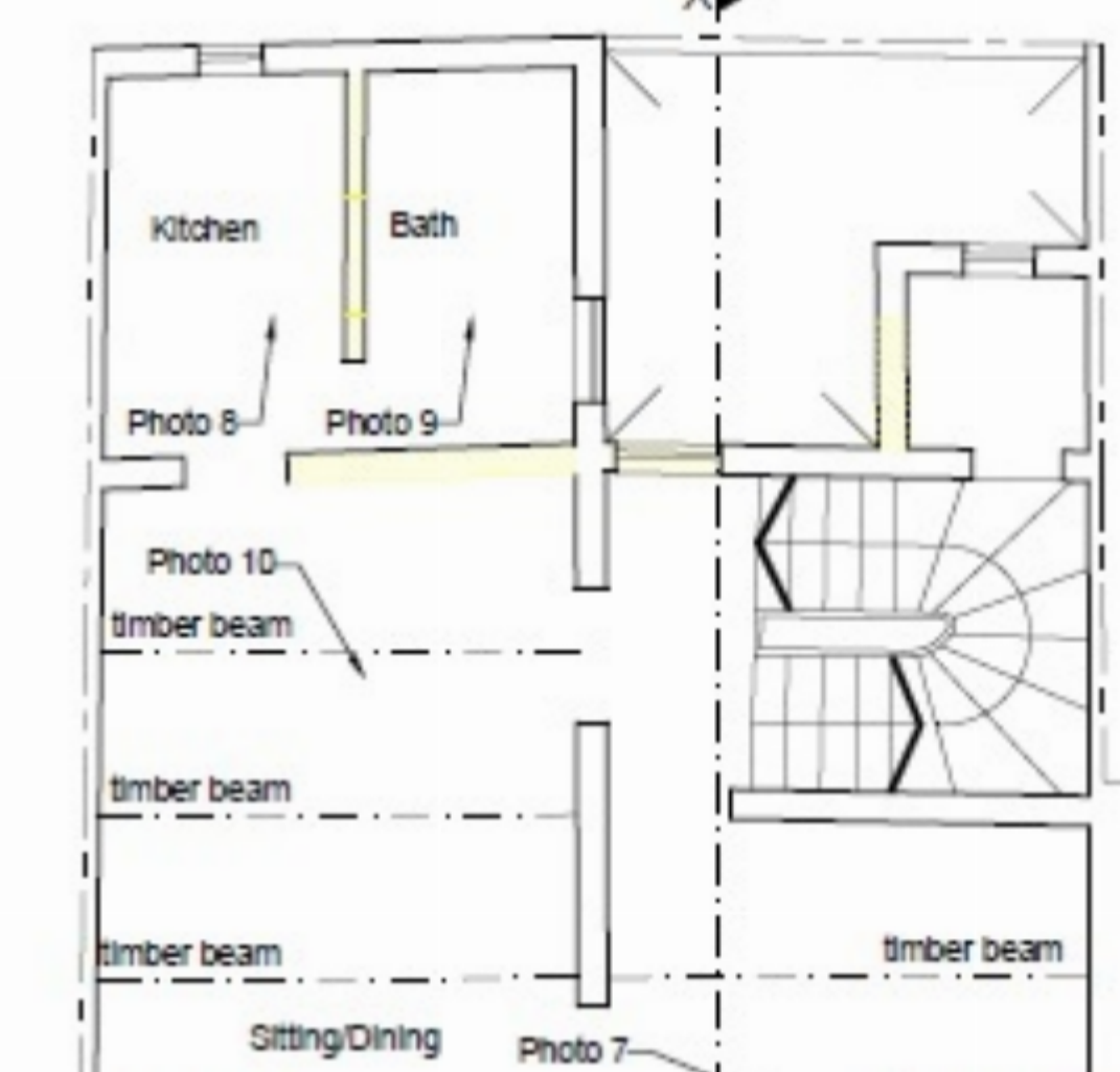
Existing First Floor SCALE 1:100
