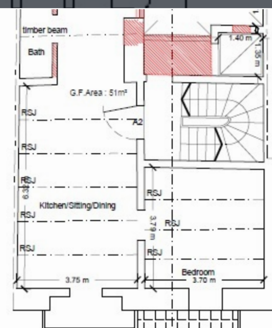
Proposed Third Floor SCALE 1:100
