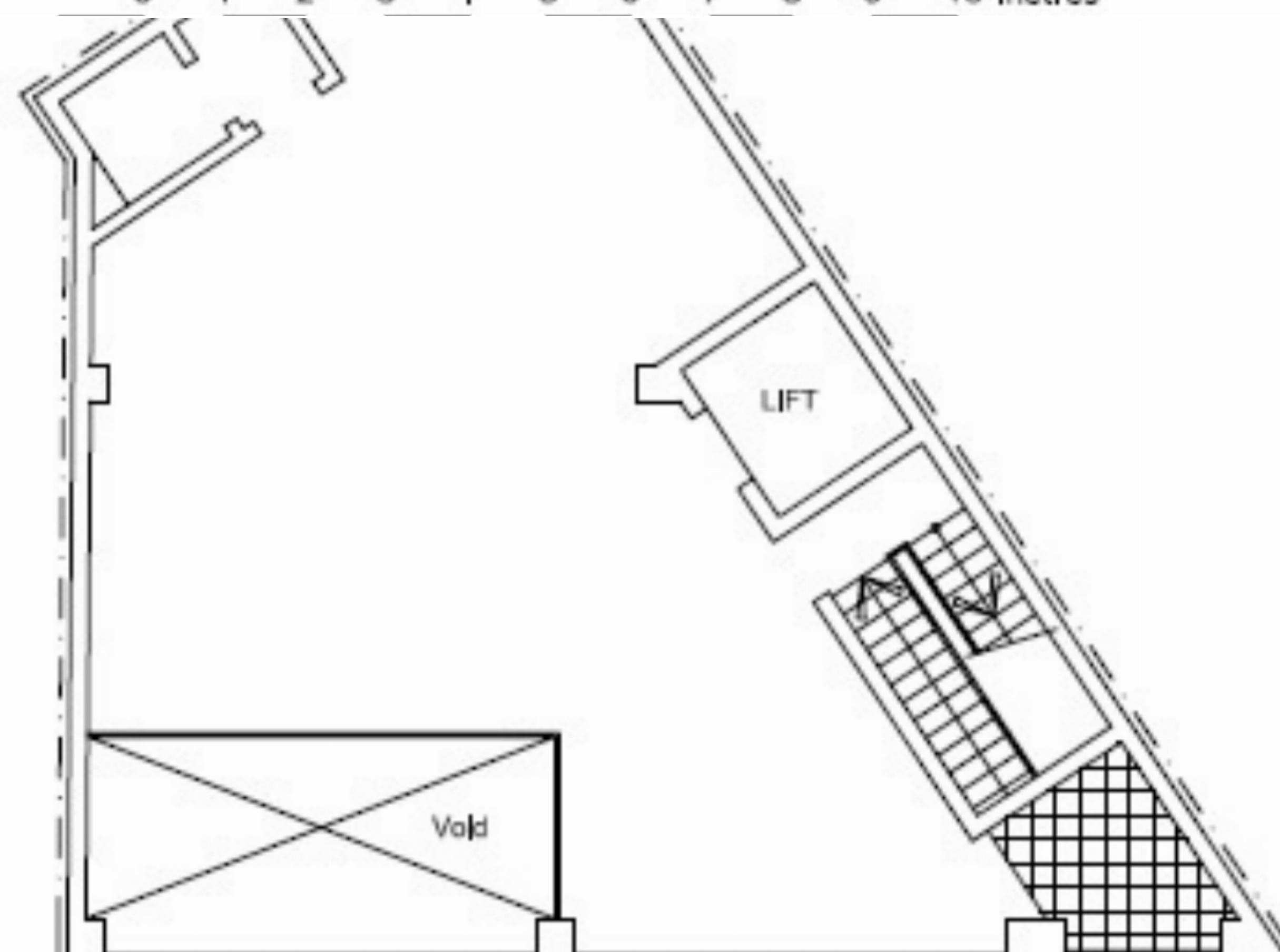
INTERMEDIATE FLOOR PLAN - as proposed
